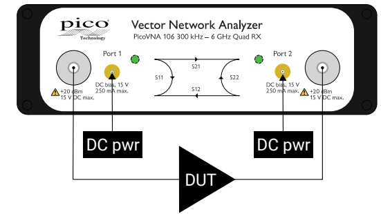
Use bias-Ts to power an active DUT
